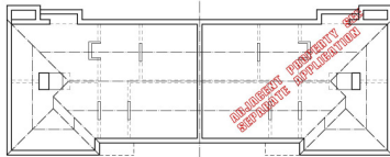
ROOF SPACE PLAN THE BUNGALOW
