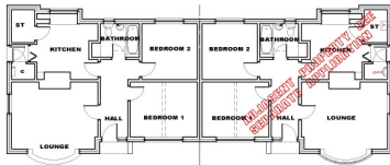
GROUND FLOOR PLAN THE BUNGALOW
